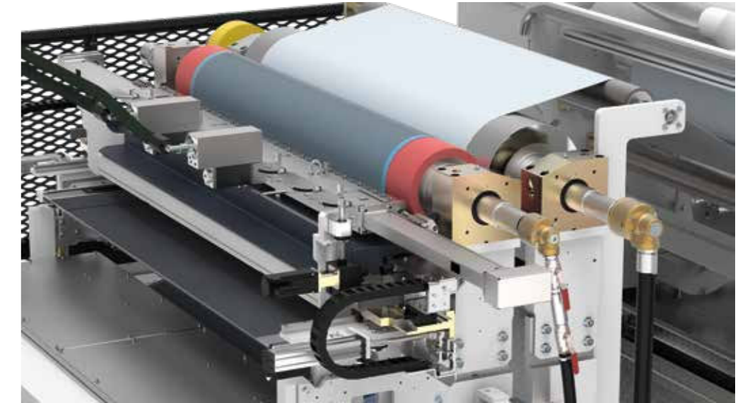
Hot-melt laminator
