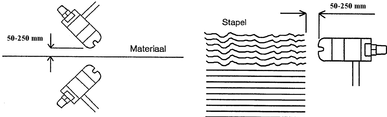
Fig. 2 Mounting example
